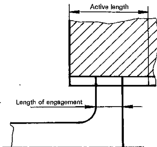
b) Hole longer than shaft
